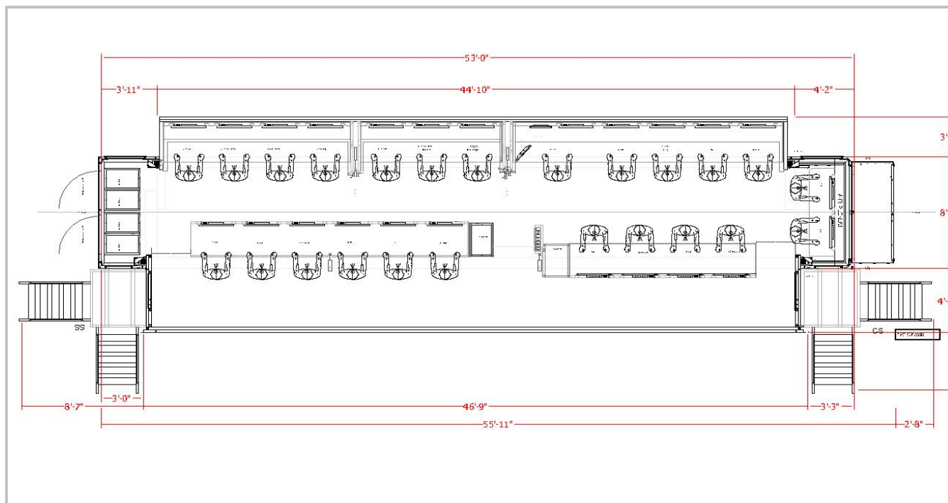
EN1D Floor Plan
