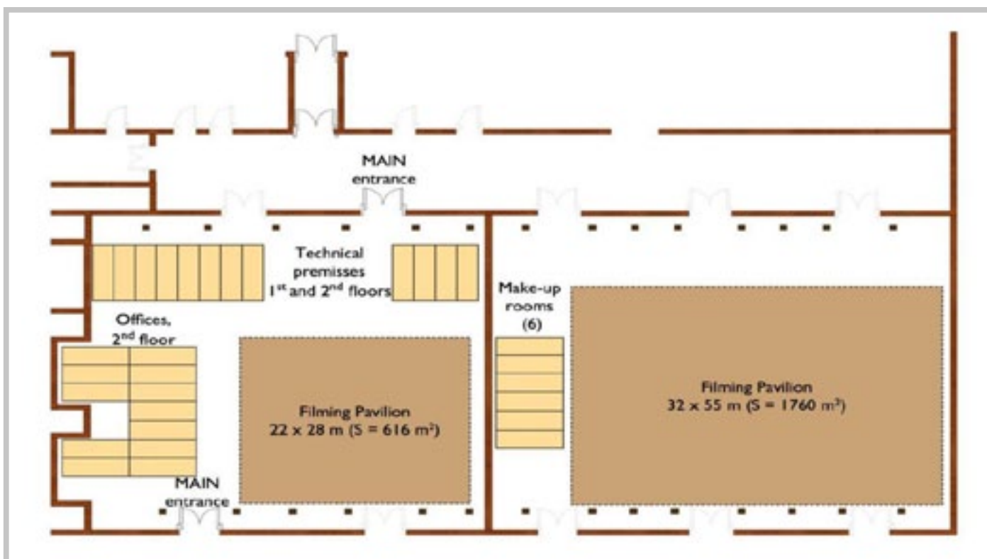
Floor Plan Filming Pavilion
